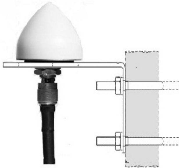
Figure 14 Antenna Mounting
