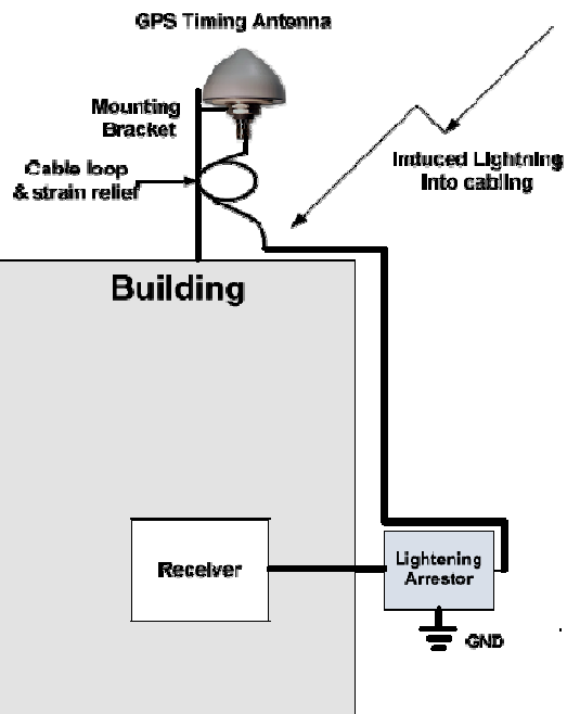
Figure 15 Antenna Mounting with Lightning Arrestor
