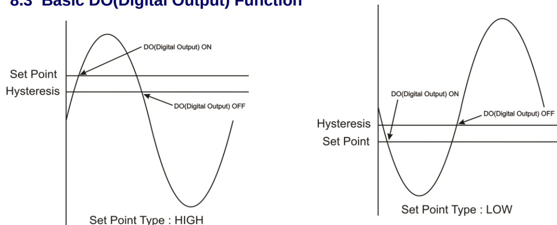
Figure 21 Basic DO(Digital Output) Function
